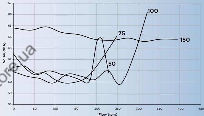
Noise Levels
