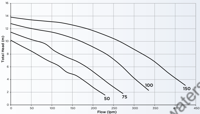
Flow Curves
