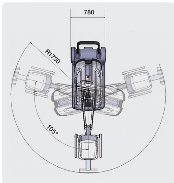
LIFT DIMENSION
